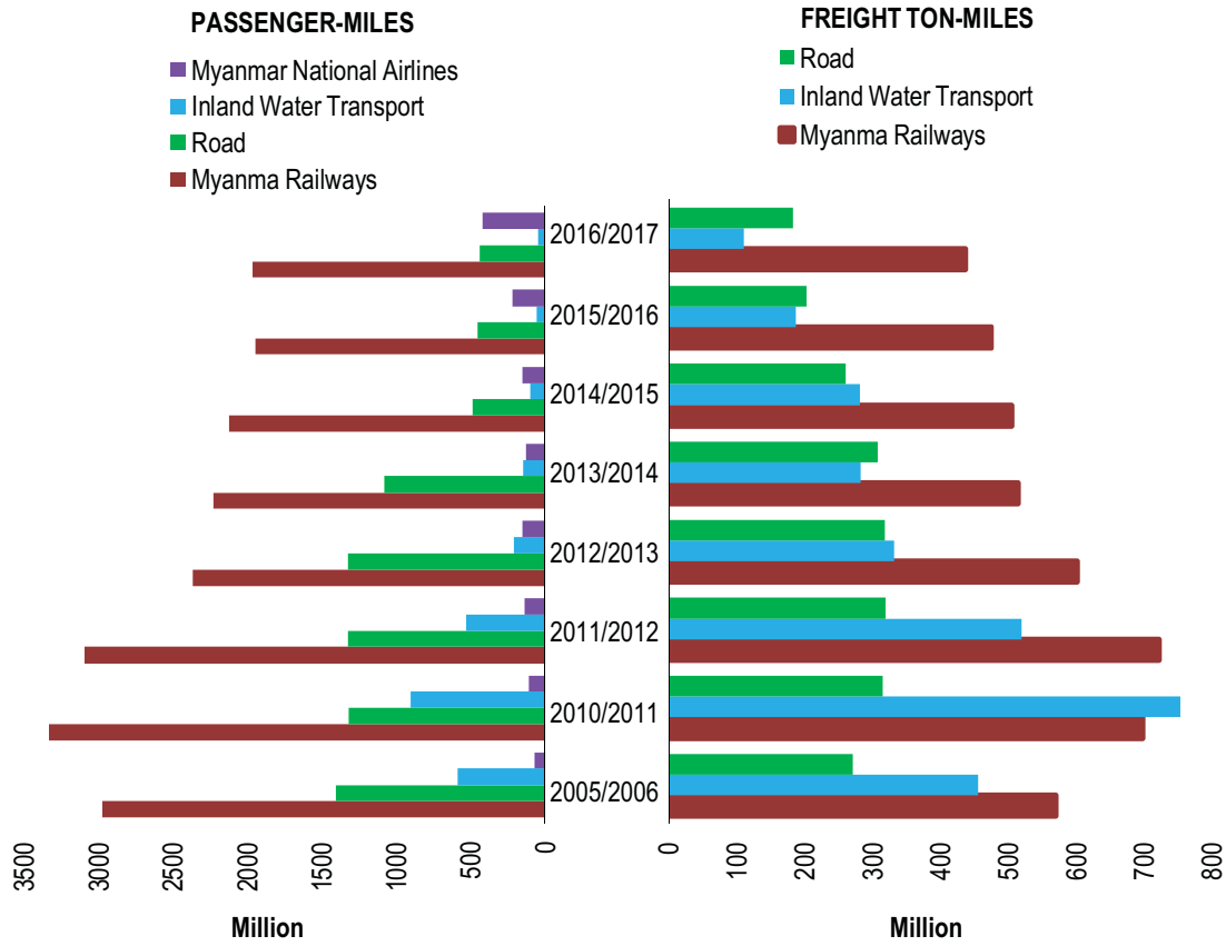
FIGURE 15.1 VOLUME OF PASSENGERS CARRIED AND FREIGHT TRAFFIC BY TYPES OF TRANSPORT
