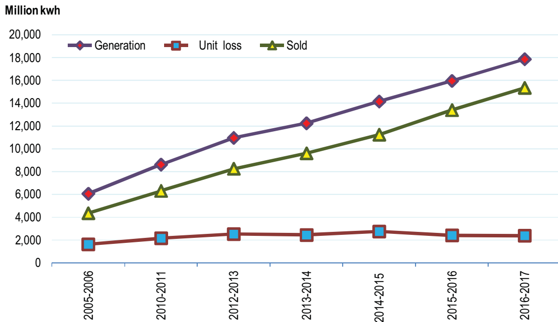
FIGURE 11.5 ELECTRIC POWER GENERATED, SOLD AND UNIT LOSS
